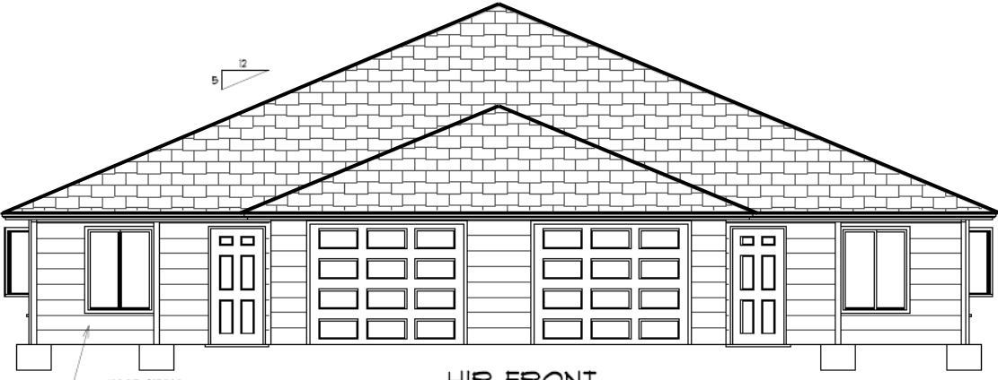
HIP FRONT ELEVATION TWO
